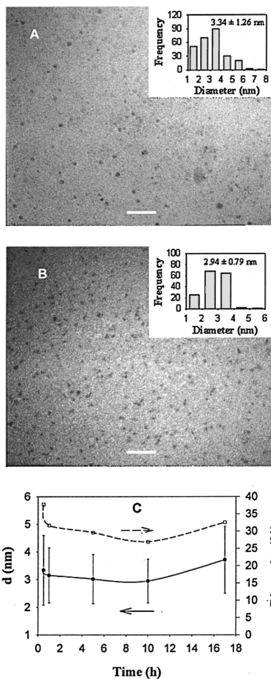
Figure 1. Representative TEM micrographs of C6–PbS (2 \times ) nanoparticles synthesized at various reaction times after the addition of \text{Na}_2\text{S} : (A) 0.5 h; and (B) 10 h. Scale bar 33 nm. Insets show the corresponding particle size histograms. (C) Variation of particle size and dispersity with reaction times.
