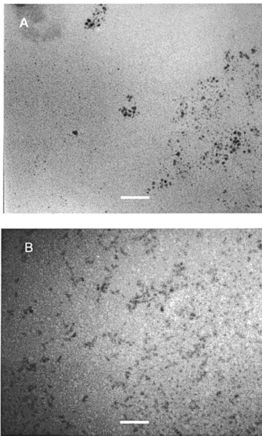
Figure 3. Representative TEM micrographs of C6–PbS nanoparticles synthesized at various C6SH/Pb ratios: (A) 0.5x; and (B) 4x scale bar 33 nm. The overall results are summarized in Table 1.
