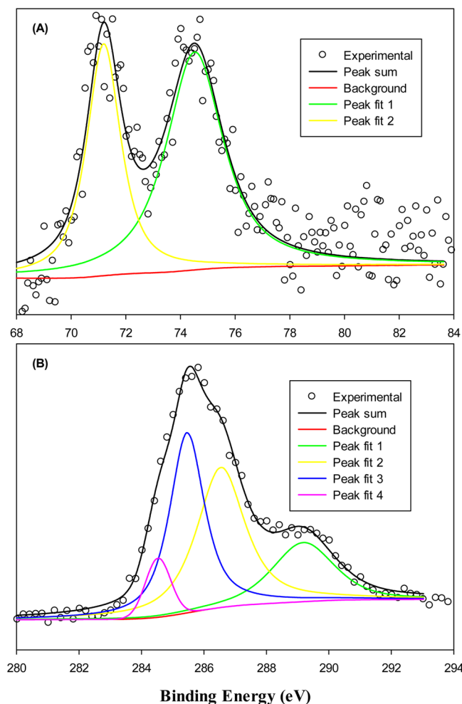
Figure 3. XPS survey spectra of the (A) Pt4f and (B) C1s electrons of the Pt/G nanoparticles. Symbols are experimental data and lines are deconvolution fits.
