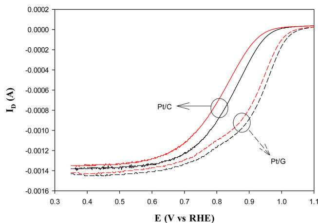
Figure 9. Polarization curves for oxygen reduction catalyzed by Pt/C (solid curves) and Pt/G (dashed curves) before (red curves) and after (black curves) 2000 potential cycles with a potential scan rate of 200 mV/s from +0.05 to +1.10 V in O 2 -saturated 0.1 M HClO 4 . Electrode rotation rate: 1600 rpm. Other experimental conditions were the same as in Figure 5.
