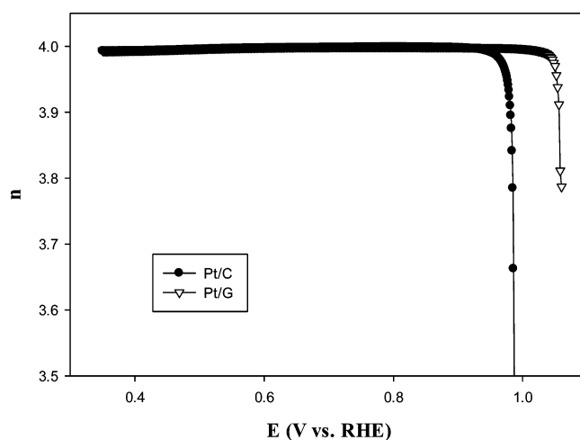
Figure 6. Variation of the number of electron transfer ( n ) in oxygen reduction with electrode potential. Symbols are experimental data calculated from the RRDE voltammograms at 2500 rpm in Figure 5 by using eq 1.
