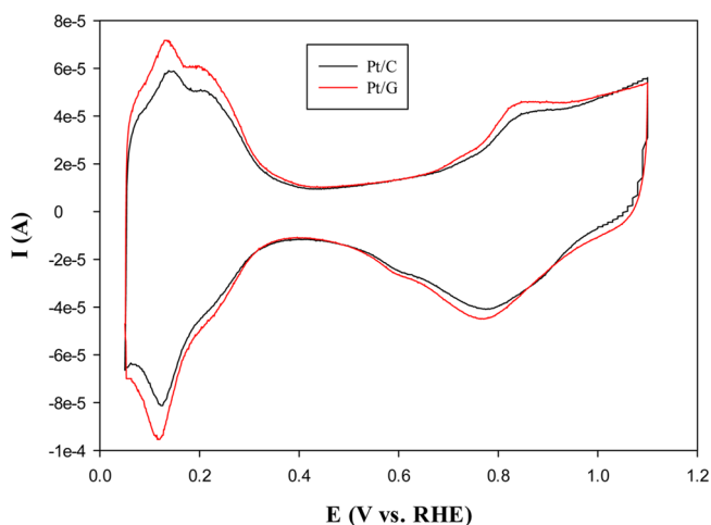
Figure 4. Cyclic voltammograms of a glassy carbon electrode (diameter 5.61 mm) loaded with Pt/G and Pt/C nanoparticle catalysts in a nitrogen-saturated 0.1 M HClO 4 solution. Metal loading was 12.1 μg for both nanoparticles. Potential sweep rate 20 mV/s.
