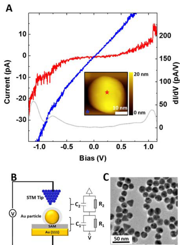
Figure 1. (A) I - V measurement of a P20 NP (see inset for its image) at tip-NP separation of 0.03 nm (red curve). An I - V measurement of the surrounding SAM is displayed in the same plot for comparison (tip-SAM separation 0.08 nm, blue curve). Red and blue stars indicate the locations above which the I - V curves were acquired for the NP and SAM, respectively. (B) Schematic illustration (left) of the SET measurements using STM imaging and spectroscopy, displayed with the corresponding equivalent circuit and the double-barrier tunneling junction (DBTJ) model (right). (C) TEM image of P20 NPs, representing the characteristic distribution of the particle size.
