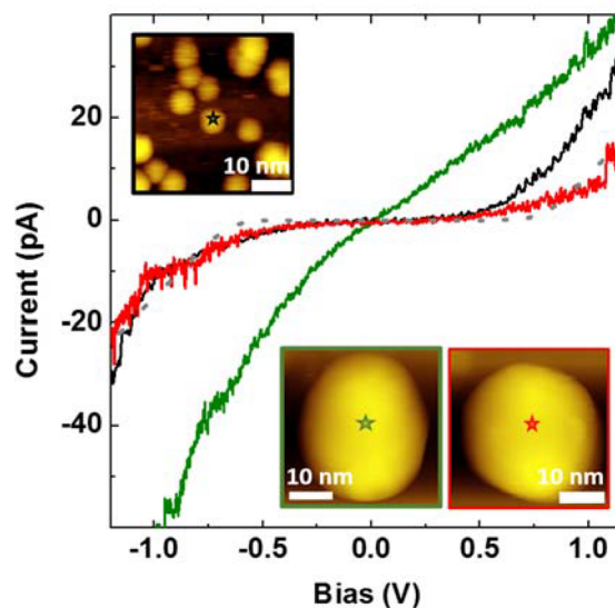
Figure 2. STS I - V characteristics of a single P20 NP (red), C20 NP (green), and S1.5 NP (black) obtained at tip-NP separations of 0.03 , 0.03 , and 0.12 nm, respectively. Insets are STM images of the NPs, where the red, green, and black stars indicate the locations above which the I - V curves were acquired for P20, C20, and S1.5 NPs, respectively. The lateral dimension in the STM images appears larger than 20 nm due to tip convolution effects. 30,31 Fitting (gray dashed line) of the I - V curve of the P20 NP based on the DBTJ model is shown in the same plot.
