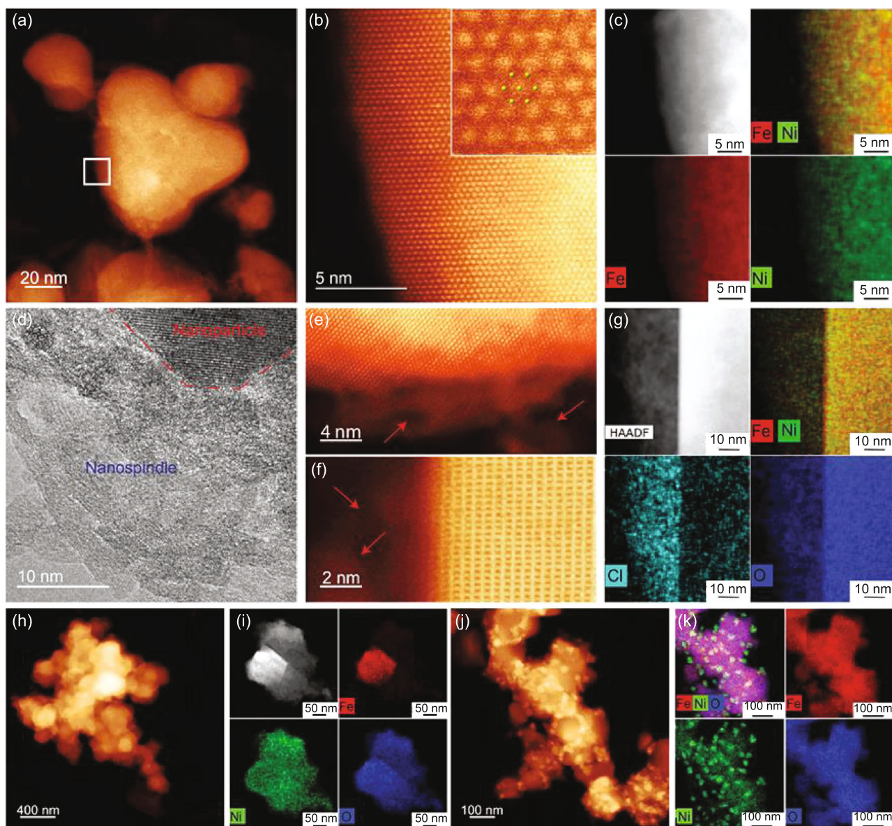
FIGURE 2: Electron microscopic studies of FeNi spinel oxides. (a) High-angle annular dark-filed scanning transmission electron microscopy (HAADF-STEM) image showing the morphology of FeNiO-250-4. (b) Atomic-resolution HAADF-STEM image and an enlarged image (inset) corresponding to the boxed region in (a) acquired along the \langle 111 \rangle zone axis. (c) High-resolution energy-dispersive spectroscopy (EDS-) based elemental maps of Fe and Ni in a FeNiO-250-4 particle, which features a FeNi spinel structure with no FeNi phase segregation. (d) High-resolution TEM (HRTEM) image of nanospindles in FeNiO-250-4. (e, f) HAADF-STEM images of nanospindles on the edge of FeNiO-250-4 (low-contrast regions), as highlighted by red arrows. (g) EDS mapping images of the interface between nanospindles and nanoparticles in FeNiO NC -250-4, which show a Cl-rich surface of the nanospindles. (h) HAADF-STEM images and (i) EDS mapping images of FeNiO NC -250-4, where natural cooling leads to the formation of nanoparticles aggregates and obvious FeNi phase segregation. (j) HAADF-STEM and (k) EDS mapping image of FeNiO-250-16, where prolonged heating (higher temperature) leads to the formation of a significant amount of metallic Ni nanoparticles on the FeNi spinel.
